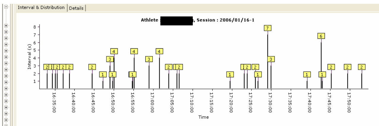
Figure 4: Sprints performed
