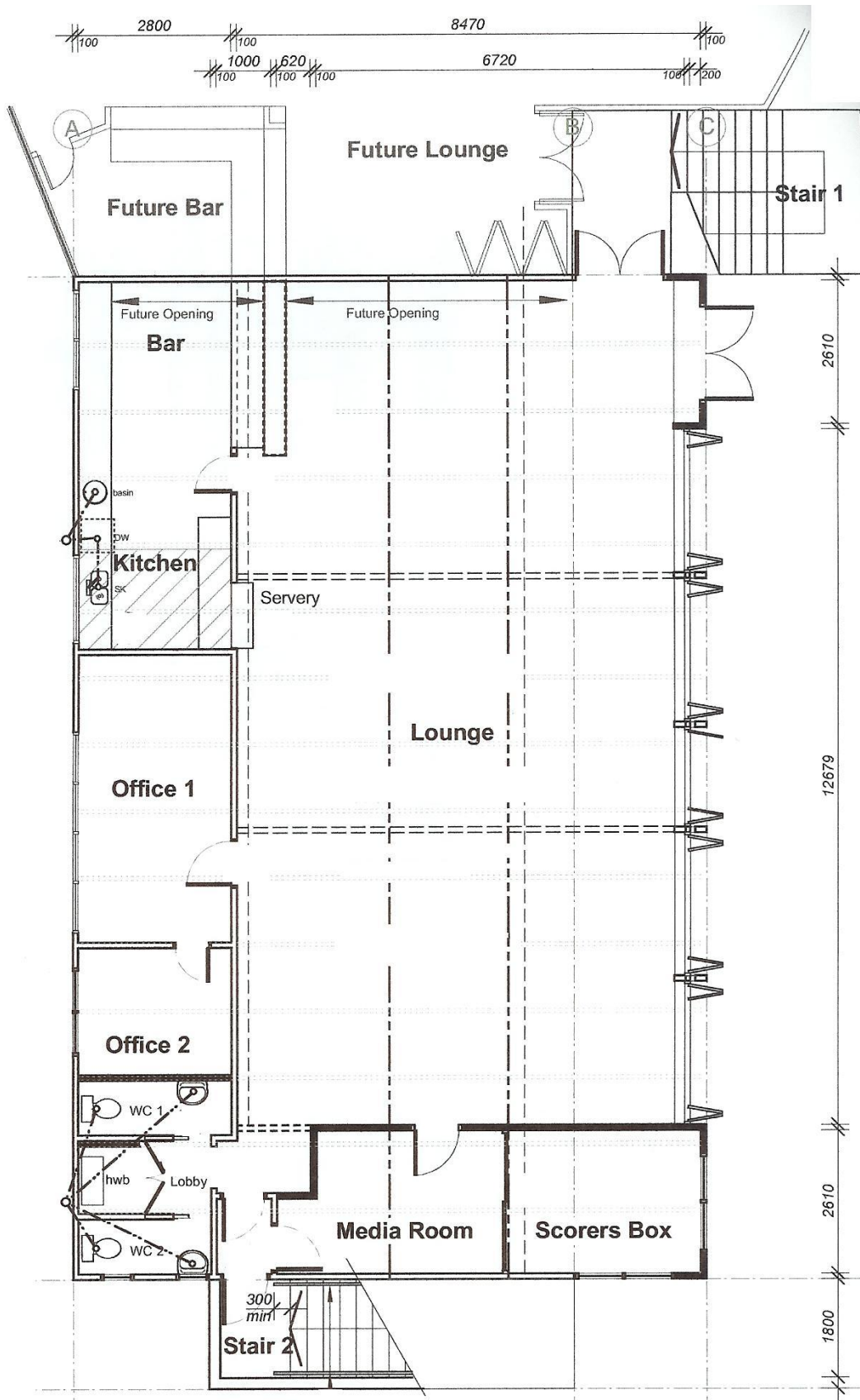
Proposed Upper Plan Pavillion
