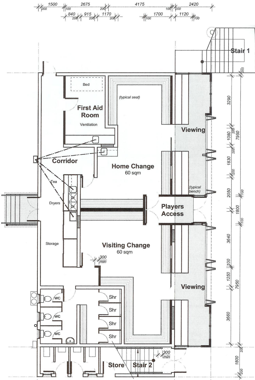
Proposed Ground Plan Pavilion
